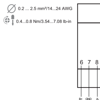
Fig. 8 RS485 port
